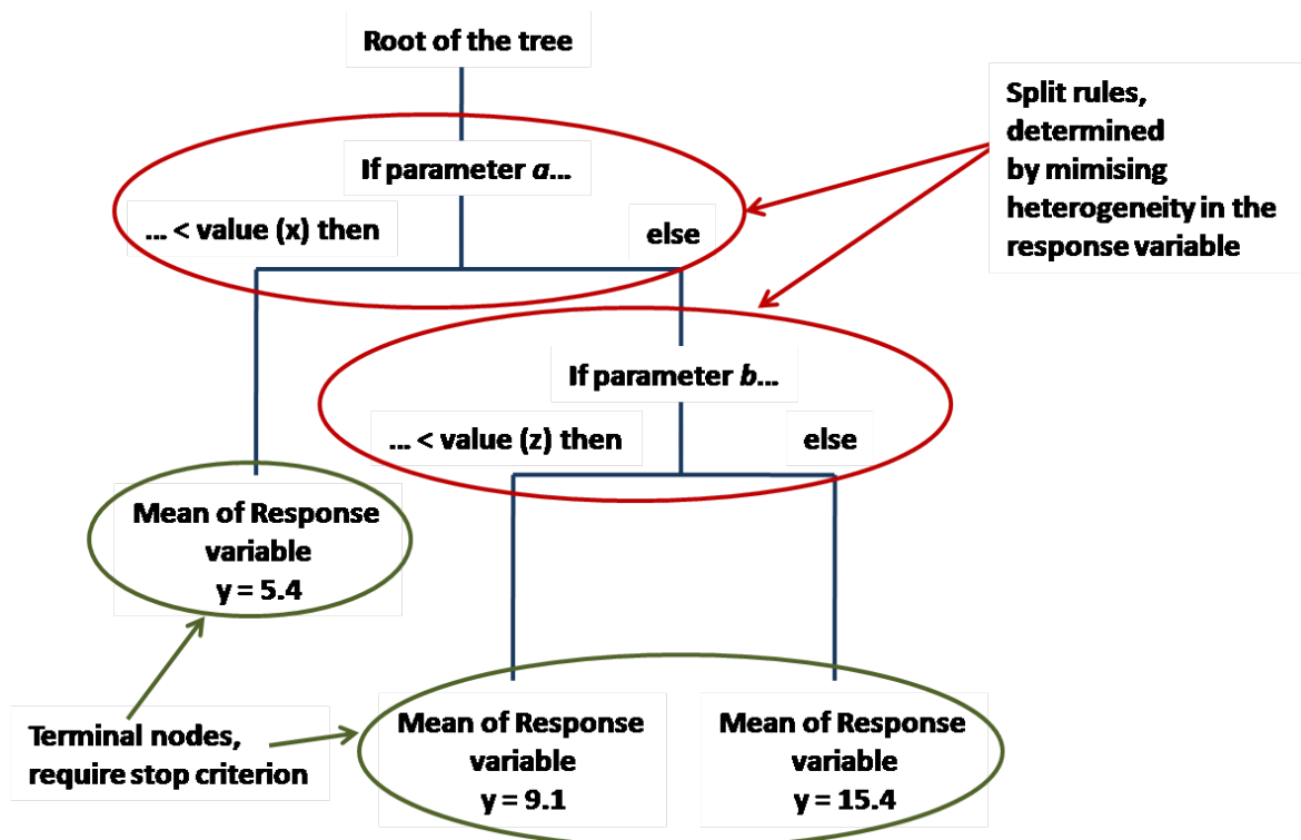
Figure 29: Sketch of a simple regression tree to illustrate the mentioned technical terms. All given numbers are exemplary without true background data.
