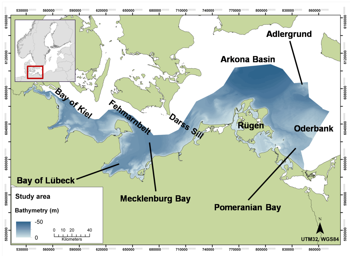
Figure 4: Study area displaying the location of sea areas frequently mentioned in the text.
