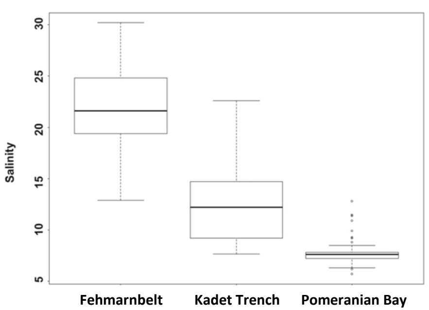
Figure 24: Boxplots showing the different salinity ranges in the three areas
