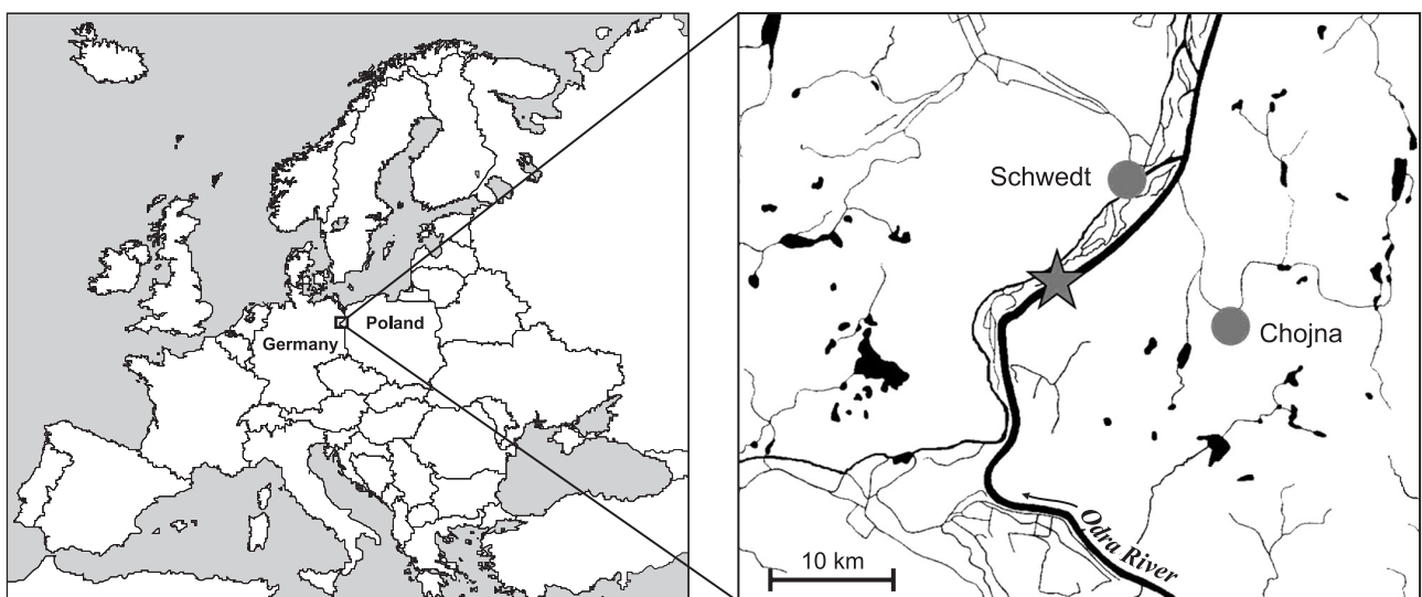
Fig. 2. Investigation area of northern Germany. The sampling station in the Oder River near Stützkw is indicated by a star
