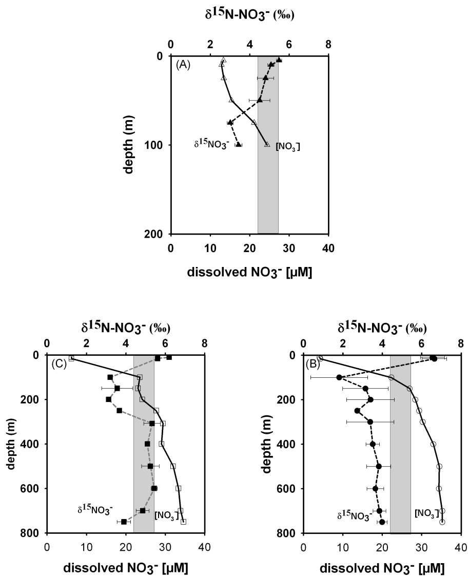
Figure 4.3: Depth profile of \text{NO}_3^- concentrations and \delta^{15}\text{N-NO}_3^- values for the Eastern tropical North Atlantic stations 244 (solid triangles), 245 (circles) and 246 (gray squares) of the POS 348 cruise. Symbols represent mean value and standard deviation of replicate analyses on individual \delta^{15}\text{N-NO}_3^- samples (except stat. 246: 400, 16 and 10 m). Grey box in \delta^{15}\text{N-NO}_3^- plot represents the range of literature values of \delta^{15}\text{N} deep \text{NO}_3^- (Knapp et al. 2005, Liu & Kaplan 1989, Sigman et al. 1997).
