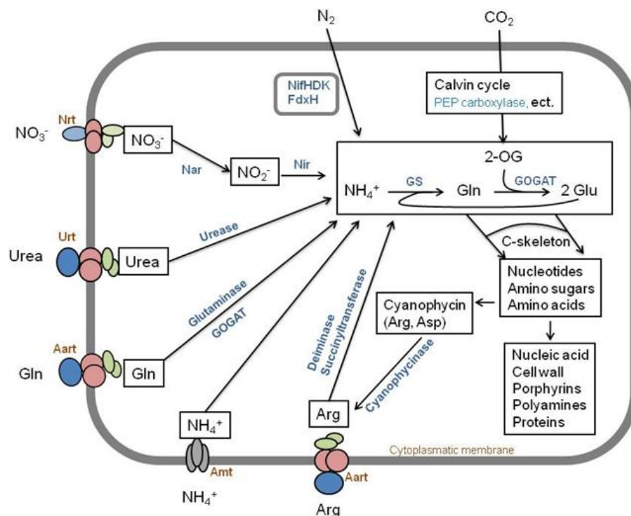
Figure 1.3: Main pathways of N assimilation in cyanobacteria (see text for further details). Abbreviations: 2-OG: 2- oxoglutarate; Arg: arginine; Asp: asparagine; Nrt: ABC-type nitrate/nitrite transporter; Urt: ABC-type urea transporter; Aart: ABC-type Amino acid transporter; Amt: ammonium permease; Nar: nitrate reductase; Nir: nitrite reductase; GS: glutamine synthase; NifHDK: nitrogenase complex; FdxH: heterocyst-specific ferredoxin; PEP carboxylase: phosphoenolpyruvate carboxylase. Nitrogenase and FdxH are boxed indicating that in some cyanobacteria N 2 fixation takes place in heterocysts. Figure adapted from Flores & Herrero (1994 and 2005).
