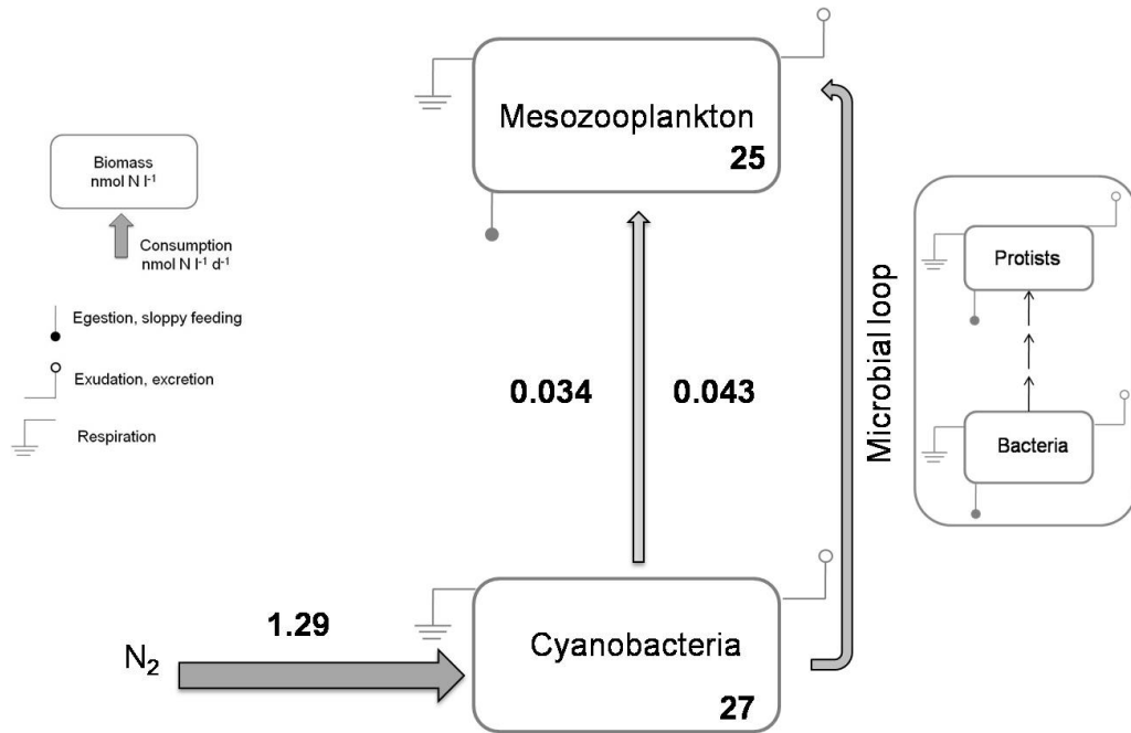
Figure 4.8: Idealized N budget using in situ abundance of mesozooplankton and the determined average N incorporation rates from Table 4.3. The numbers in the box are the mean standing stock (nmol N l -1 ). Numbers next to the arrow are fluxes of N (nmol N l -1 d -1 ). Thicknesses of arrows are roughly proportional to the N flux. Egestion, sloppy feeding, exudation, excretion and respiration were not quantified and are only used to illustrate loss terms for the single trophic positions.
