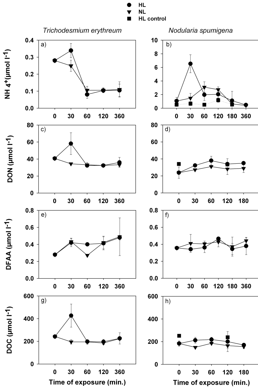
Figure 2.5: Time dependent variability of \text{NH}_4^+ (a,b), DON (c,d), DFAA (e,f) and DOC (g,h) concentration for Trichodesmium erythraeum and Nodularia spumigena and the two light regimes, respectively: high light (HL, circles, 200 or 100 \mu\text{mol photons m}^{-2} \text{s}^{-1} ) vs. normal light (NL, triangle, 100 or 60 \mu\text{mol photons m}^{-2} \text{s}^{-1} ). HL control (square) treatments with no Nodularia spumigena present. Symbols represent the mean value of three replicates and standard deviation.
